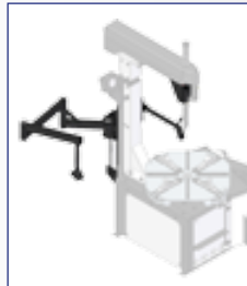
20011133 PRESS SYSTEM Bracci pneumatici premi-tallone. Pneumatic arm for bead pressing assist.
